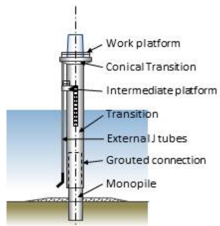
Plate 6.6 Typical Monopile
