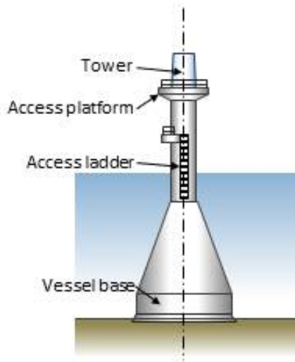
Plate 6.3 Typical Gravity Base Structure
