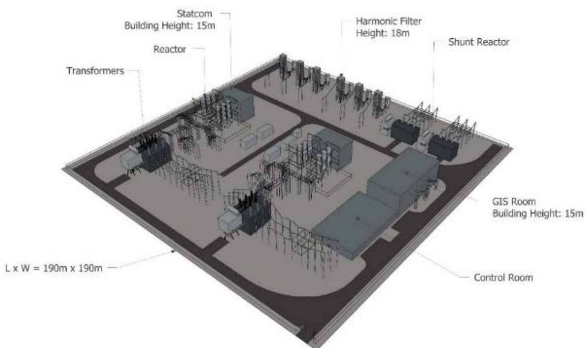
Plate 6.27 Rochdale Envelope 3D model of East Anglia TWO Onshore Substation
