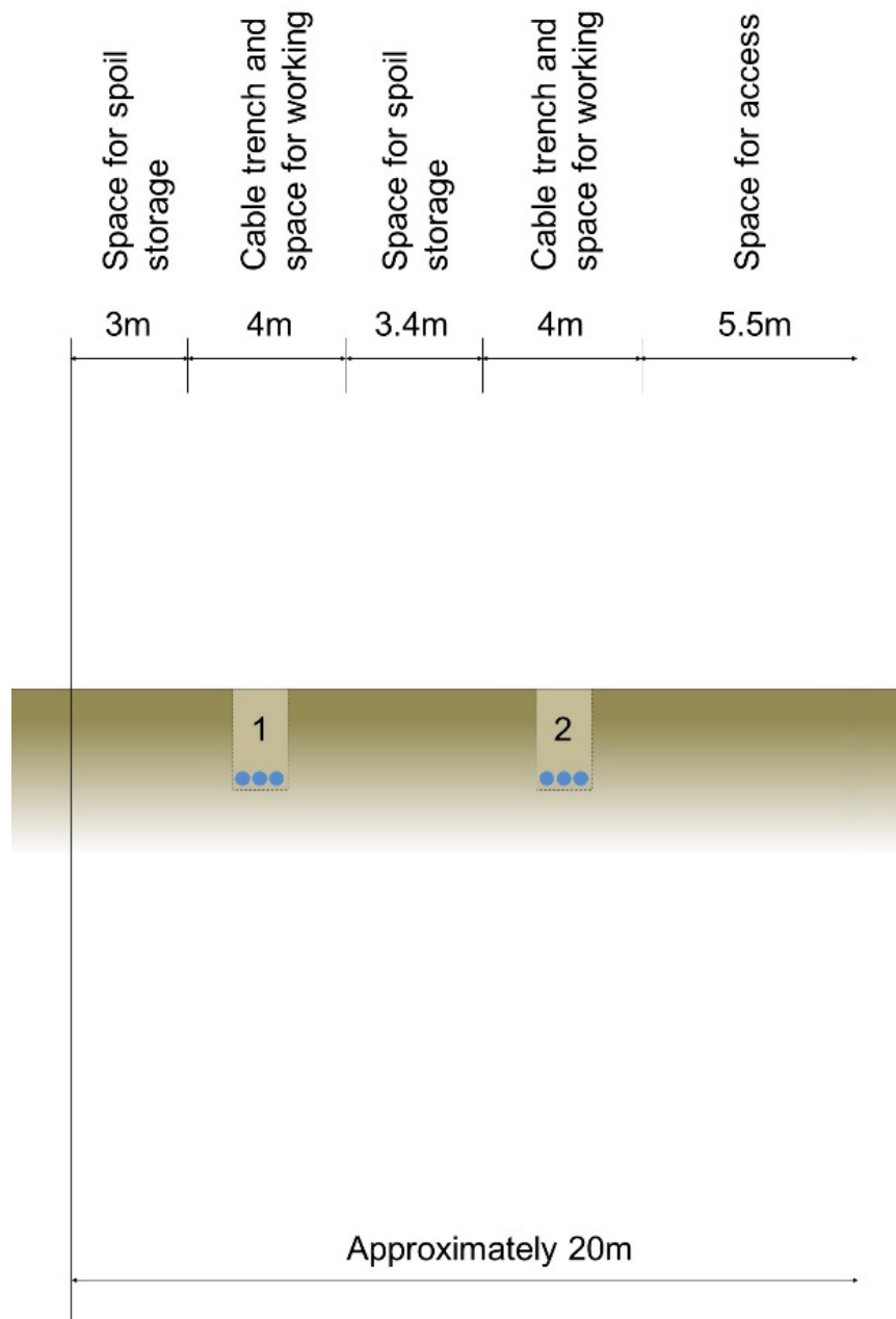
Plate 6.20 Indicative Post Construction Permanent Cable Corridor Easement
