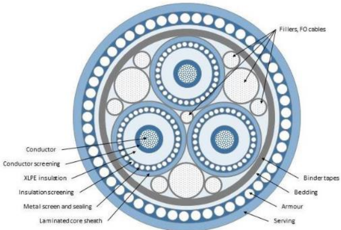
Plate 6.11 Inter-array Cables
