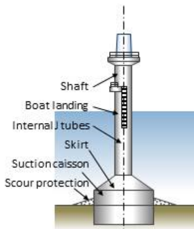
Plate 6.5 Typical Suction Caisson
