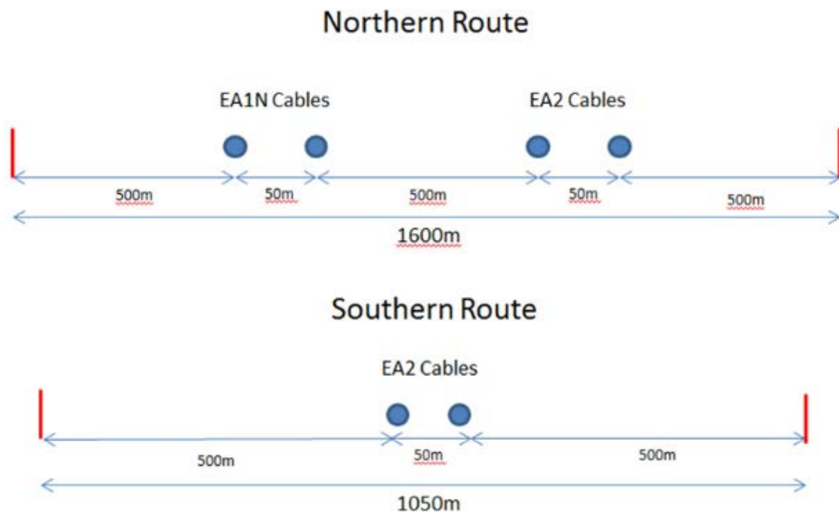
Plate 6.10 Northern Route: Indicative distances between individual export cables, within a pair, for the proposed East Anglia TWO and East Anglia ONE North projects and the indicative distance between each project's pair of export cables (500m), with 500m working width either side. Southern Route: Indicative distance between export cables with 500m working width either side.
